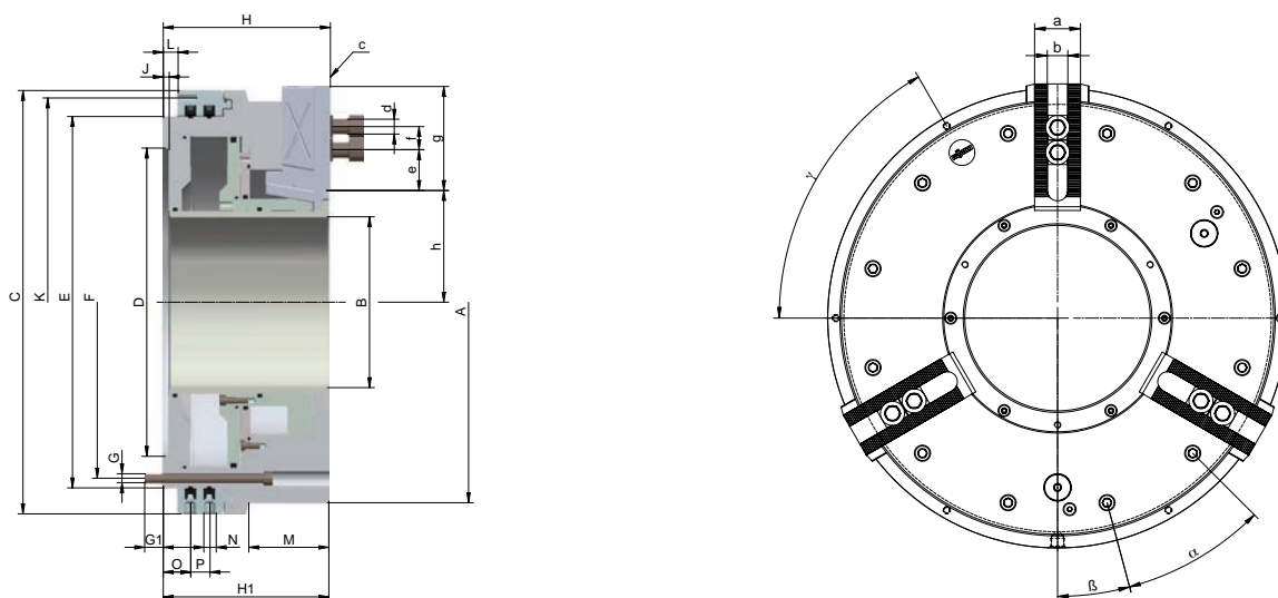
C 15 3-jaw self-contained chucks LVE, with large through-hole, max. operating pressure 8 bar, with serration Cylindrical centre mount (standard version)
