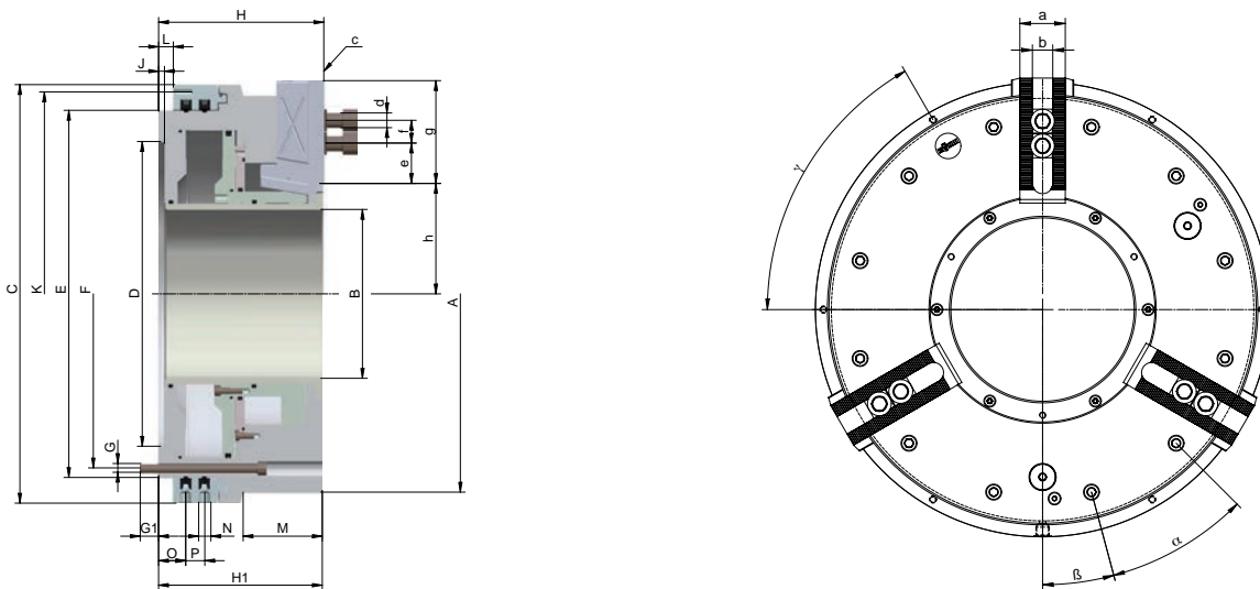
C 15 3-jaw self-contained chucks LVE, with large through-hole, max. operating pressure 8 bar, with serration Cylindrical centre mount with pressure control device for external clamping
